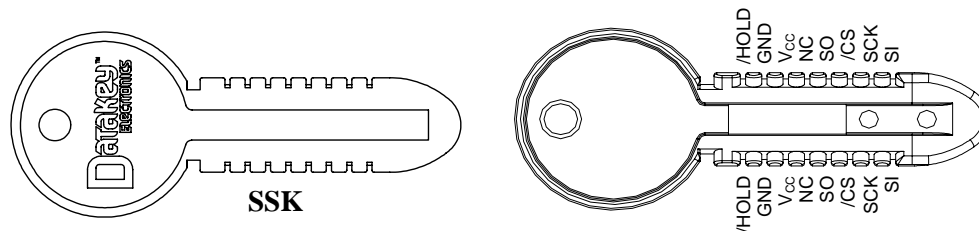
Figure 16: SSK Keys for KC4210 Keyceptacle and Key Pin Out
