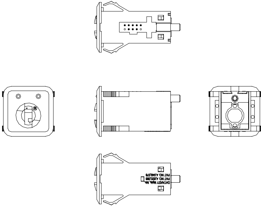
Figure 11: KC4210 Panel-Mount Keyceptacle Orthographic Drawing
