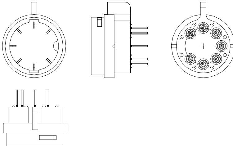
Figure 26: KSD Receptacle Orthographic Drawing
