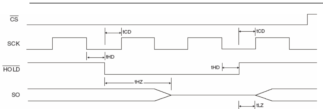
Figure 33: \overline{HOLD} Timing
